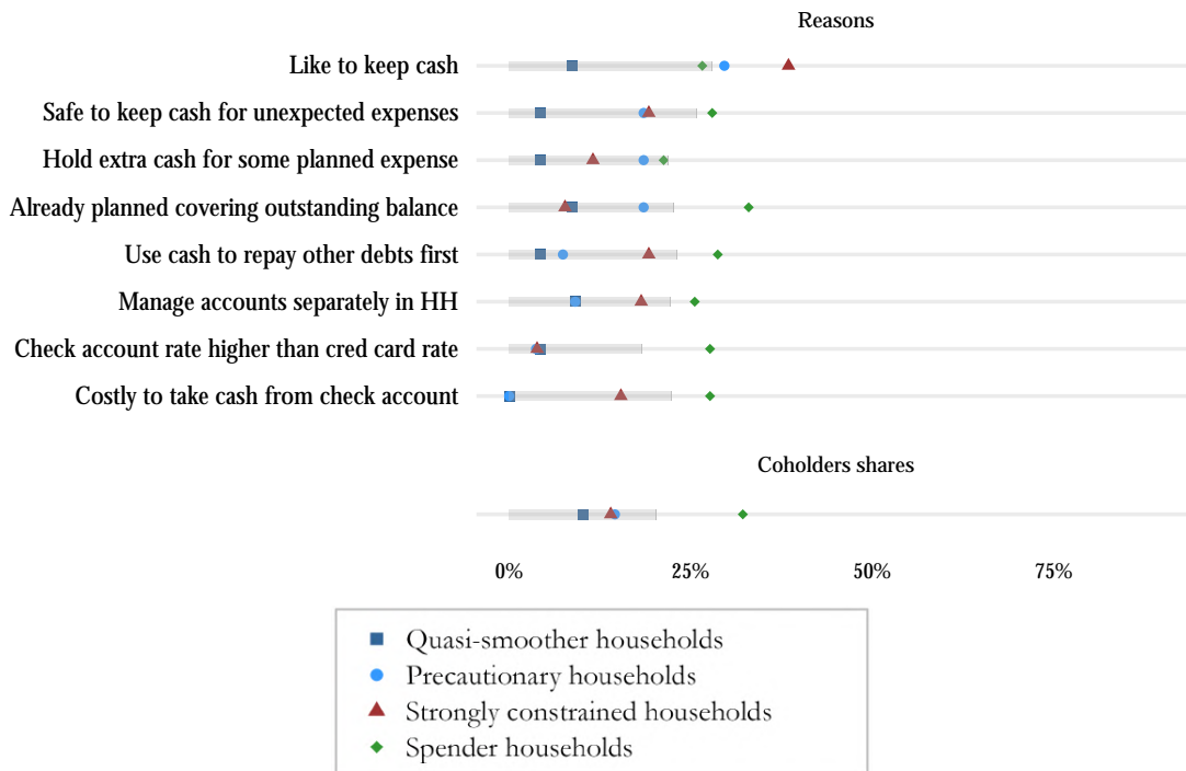
FIGURE 24: COHOLDING PUZZLE
